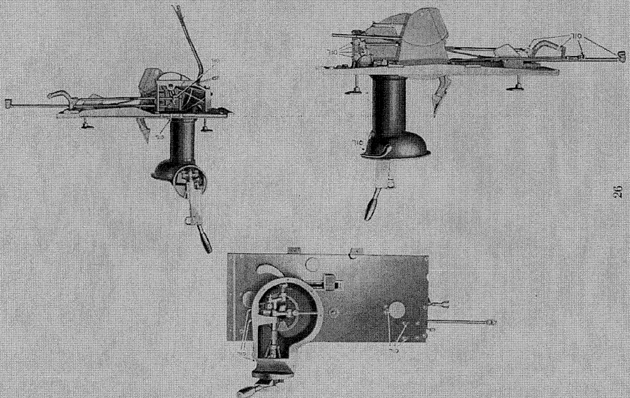
Three Views of the Pedestal Controller Mechanism
